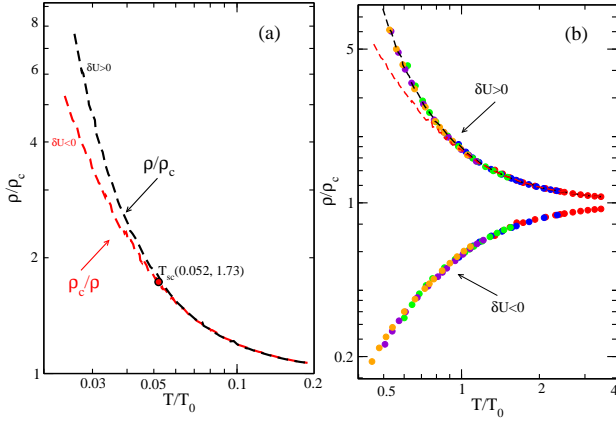
Figure 8: (a) Total scaled data (for clarity shown by single branches) exhibit reflection symmetry for T \geq T_{sc} . (b) T/T_0 -axis is rescaled by T_{sc} in such a way that T/T_0 = 1 set the boundary of quantum critical region over which the reflection symmetry of scaled curves is observed.
